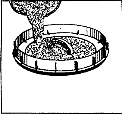
Figure 1: Set Riser Pan on floor or other suitable surface for pouring concrete. Pour concrete up to level of flat ring and insert handle.
