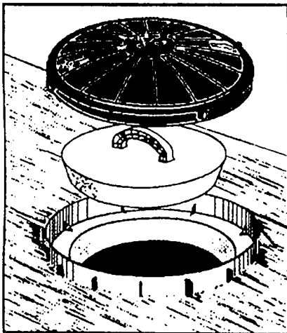
Figure 4: After concrete sets, tank is ready for a water-tight lid or stackable riser (shown in Figure 5).
