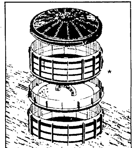
Figure 6: Riser shown cast into tank with Riser Pan, concrete lid, second Riser, and Riser Lid. *Seal with Conseal butyl rope.
