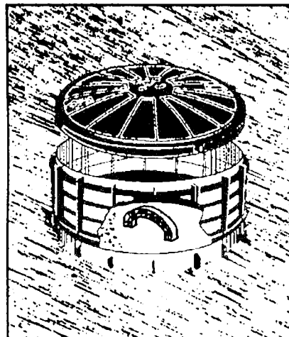
Figure 5: Riser Pan and concrete lid shown cast into tank with Riser (cutaway) and Riser Lid.
