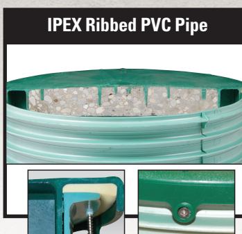
IPEX Ribbed PVC Pipe Water-TITE™ Joint Horizontal Safety Screws
