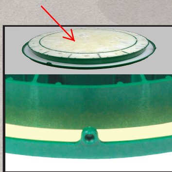
Foamed-in Permanent Polyurethane Gasket.
