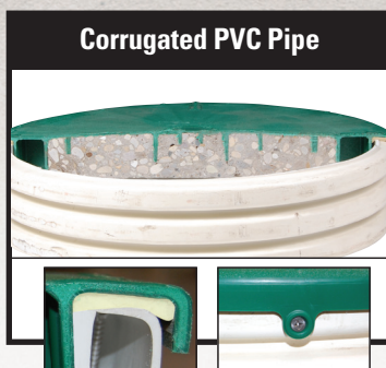
Corrugated PVC Pipe Water-TITE™ Joint Horizontal Safety Screws
